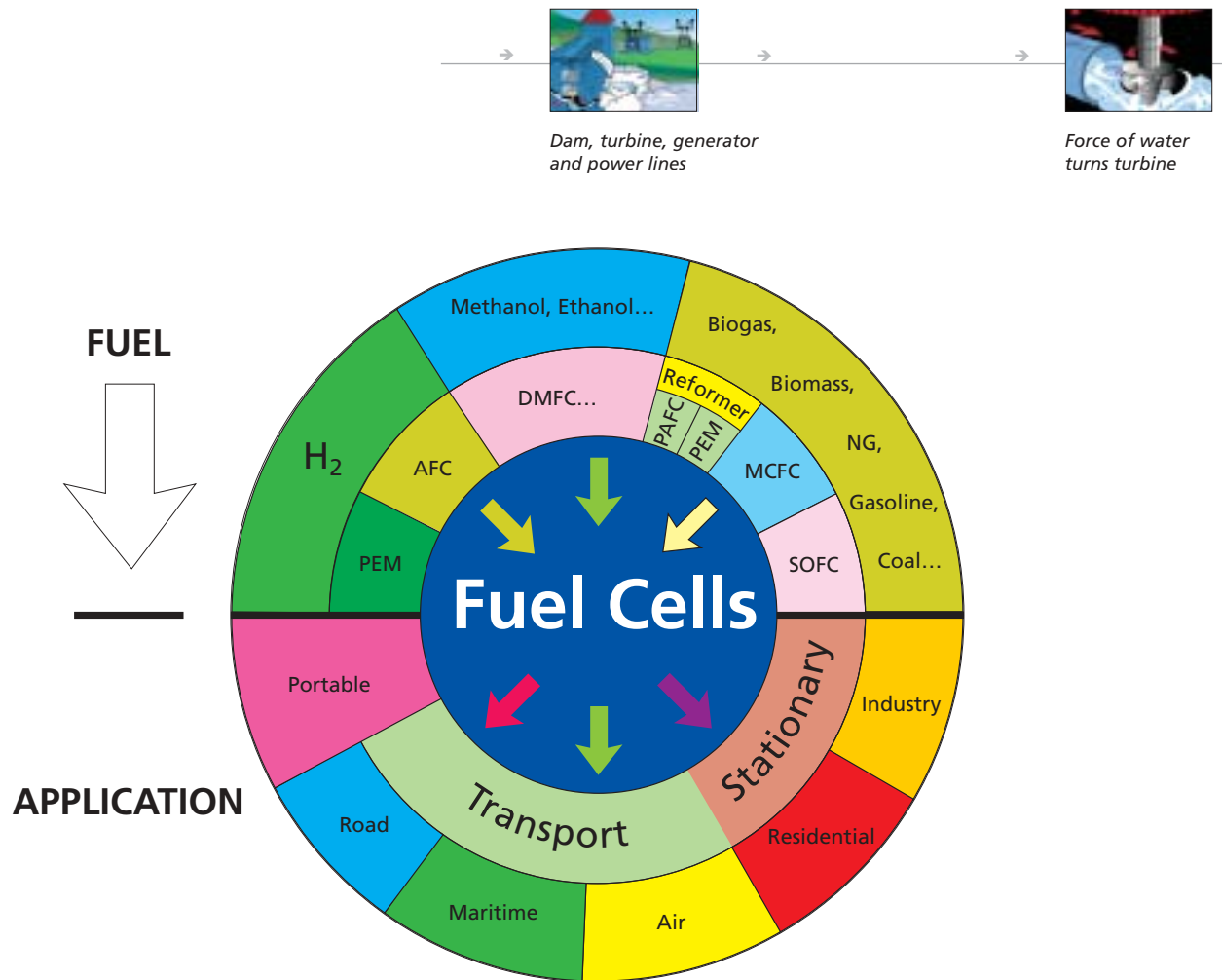
Figure 2: Fuel cell technologies, possible fuels and applications
